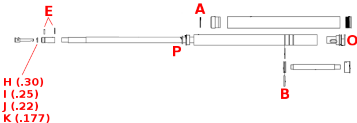
Barrel Kit (Drawing B)
